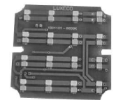
LED unit 16x LED 12V 1W white + warm white Art. nr.1333101
